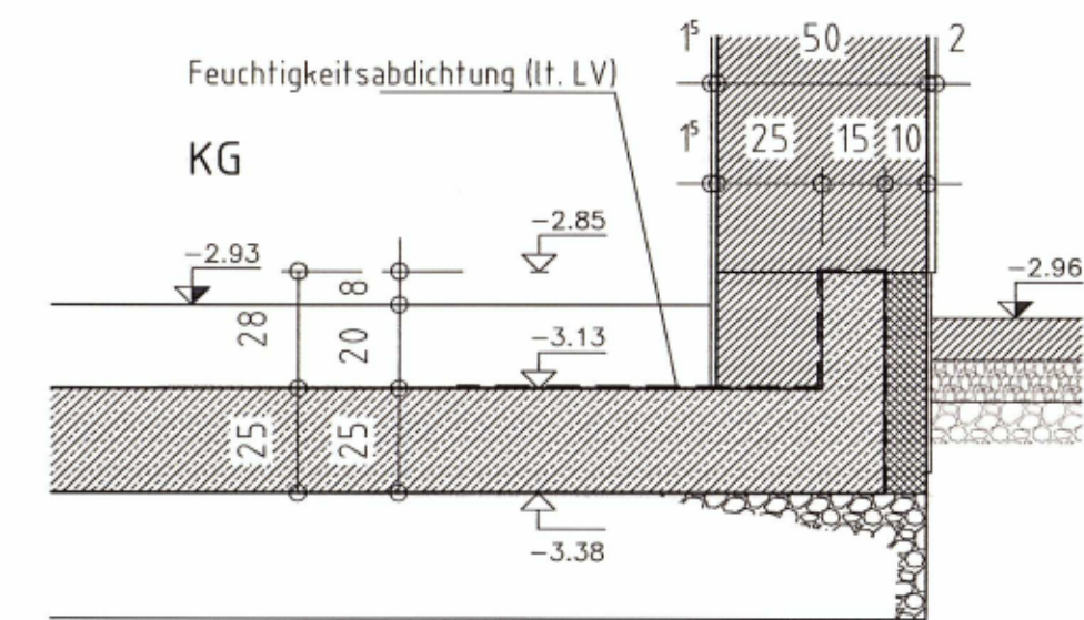
SOCKELDETAIL (KG) 1:20
